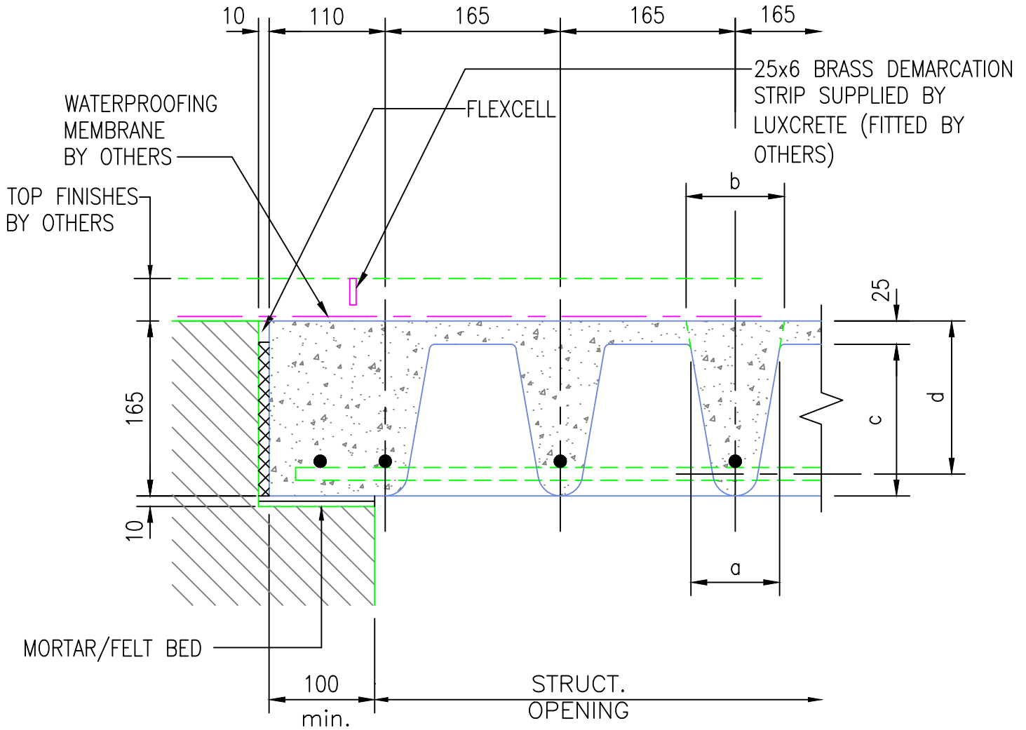
TYPICAL EDGE/CROSS SECTION
