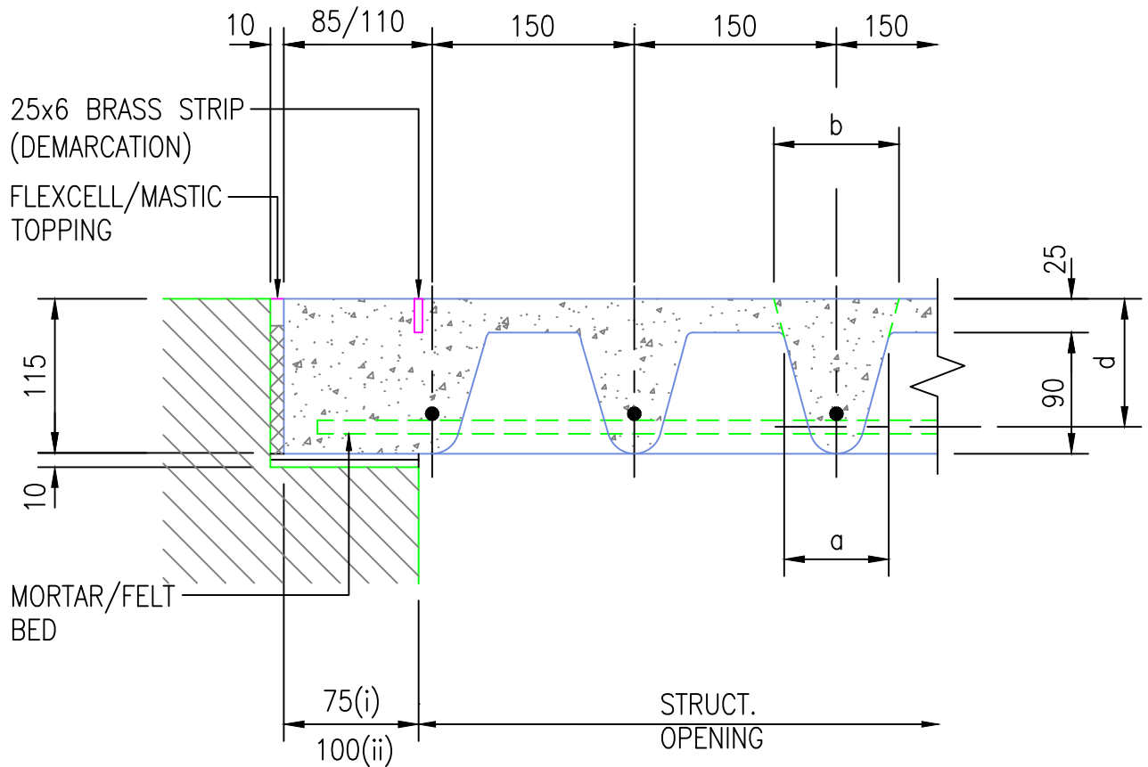
TYPICAL EDGE/CROSS SECTION
