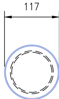
LENS PATTERN Available Clear Stippled or Prismatic (SCALE=1:5.)
